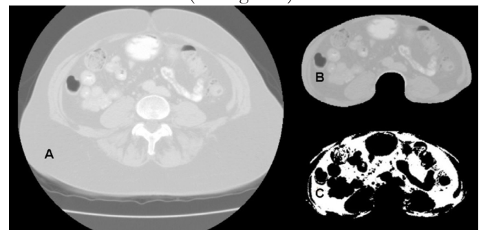
Figure 3: Segmentation process
