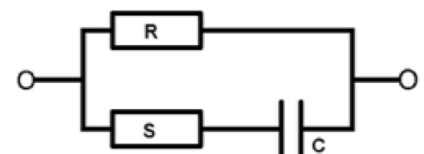
Figure 1: Equivalent circuit modeling biological tissue
